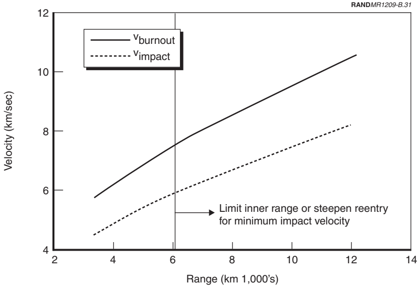
Figure B.31—Velocities for Ballistic Trajectory from Terrestrial Base with 60° Reentry Angle
