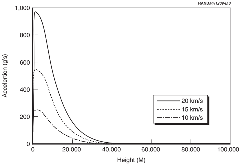
Figure B.3—Acceleration, Idealized 325-Ton Iron Spherical Meteoroid (entry at 60°)
