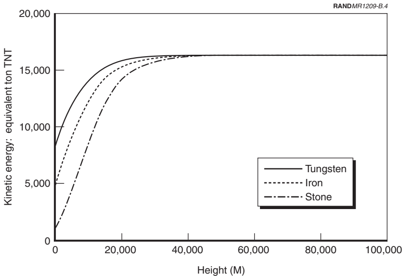
Figure B.4—Kinetic Energy, Idealized Spherical 325-Ton Meteoroids (entry at 20 km/s and 60°)
