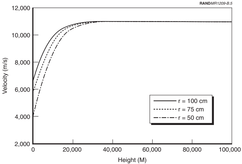
Figure B.5—Velocity, Tungsten Sphere (entry at 11 km/s)
