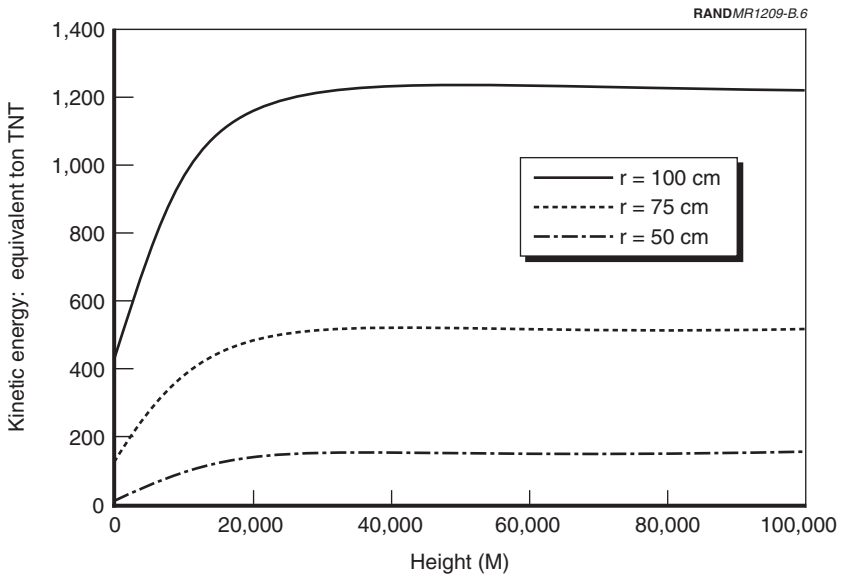
Figure B.6—Kinetic Energy, Tungsten Sphere (entry at 11 km/s)
