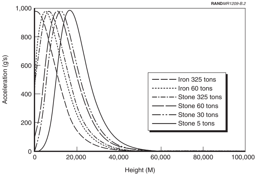
Figure B.2—Acceleration, Idealized Spherical Meteoroids (entry at 20 km/s and 60°)
