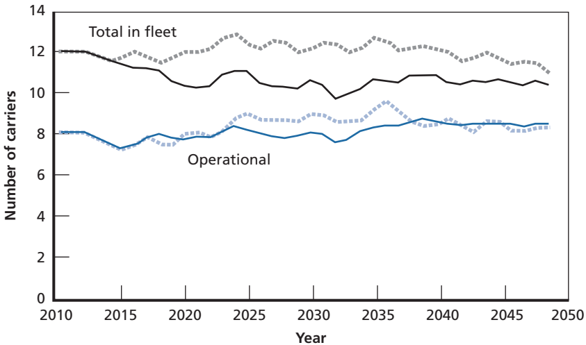
Figure 2.15 Fleet Size Sustained by 30-Month Build-New Interval and 26-Year Unrefueled Life Span
