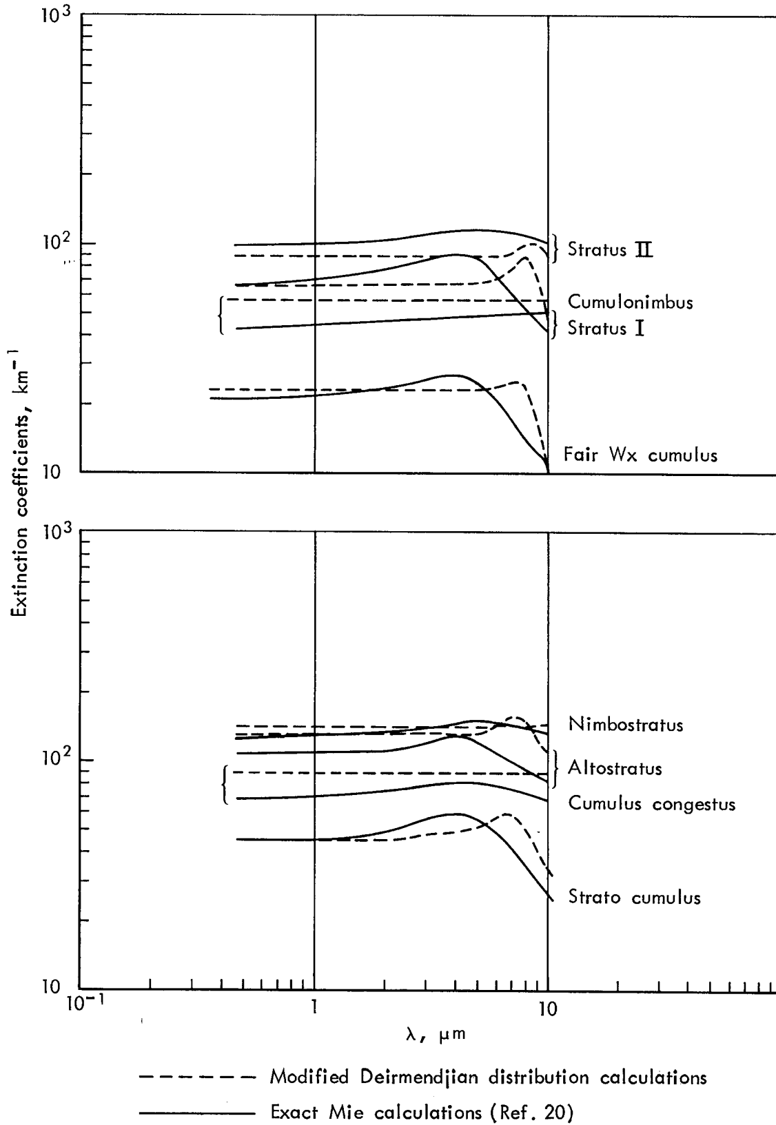
Fig.6— Calculated visible/IR extinction coefficient due to clouds
