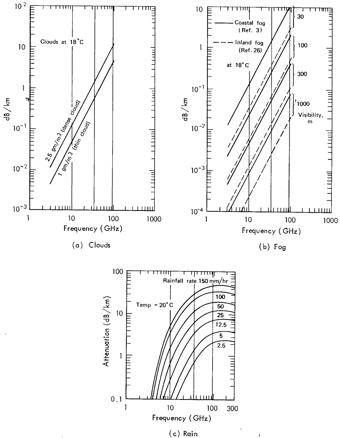
Fig. S2—Radio frequency attenuation due to clouds, fog and rain
