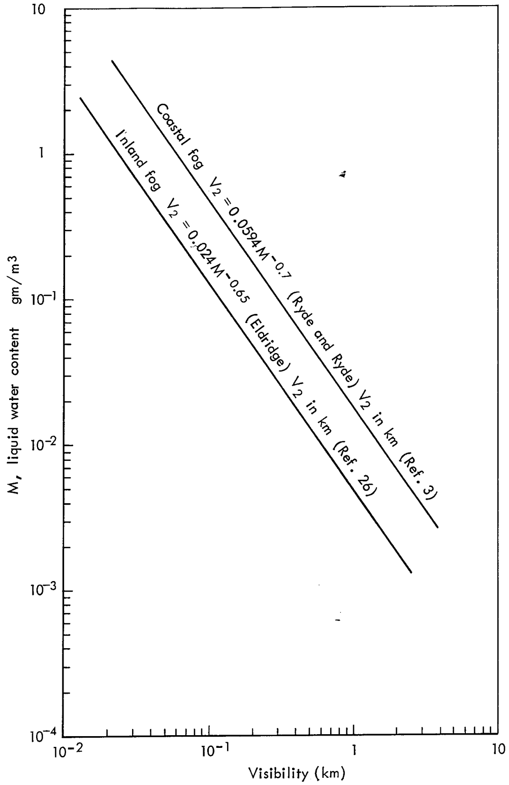
Fig. 11—Correlation of visibility in fog to liquid water content
