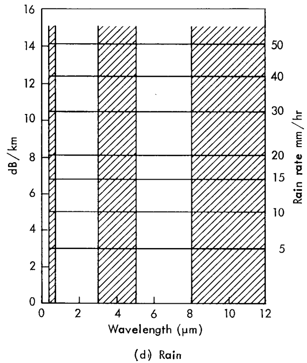
Fig. S1—Optical attenuation due to haze, fog, clouds and rain
