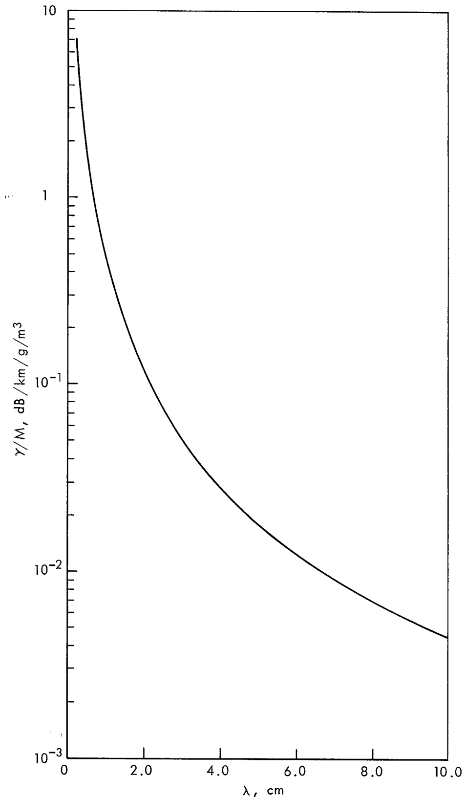
Fig. 7— Calculated attenuation coefficients by small droplets of water (e.g., clouds or fog) at 18°C
