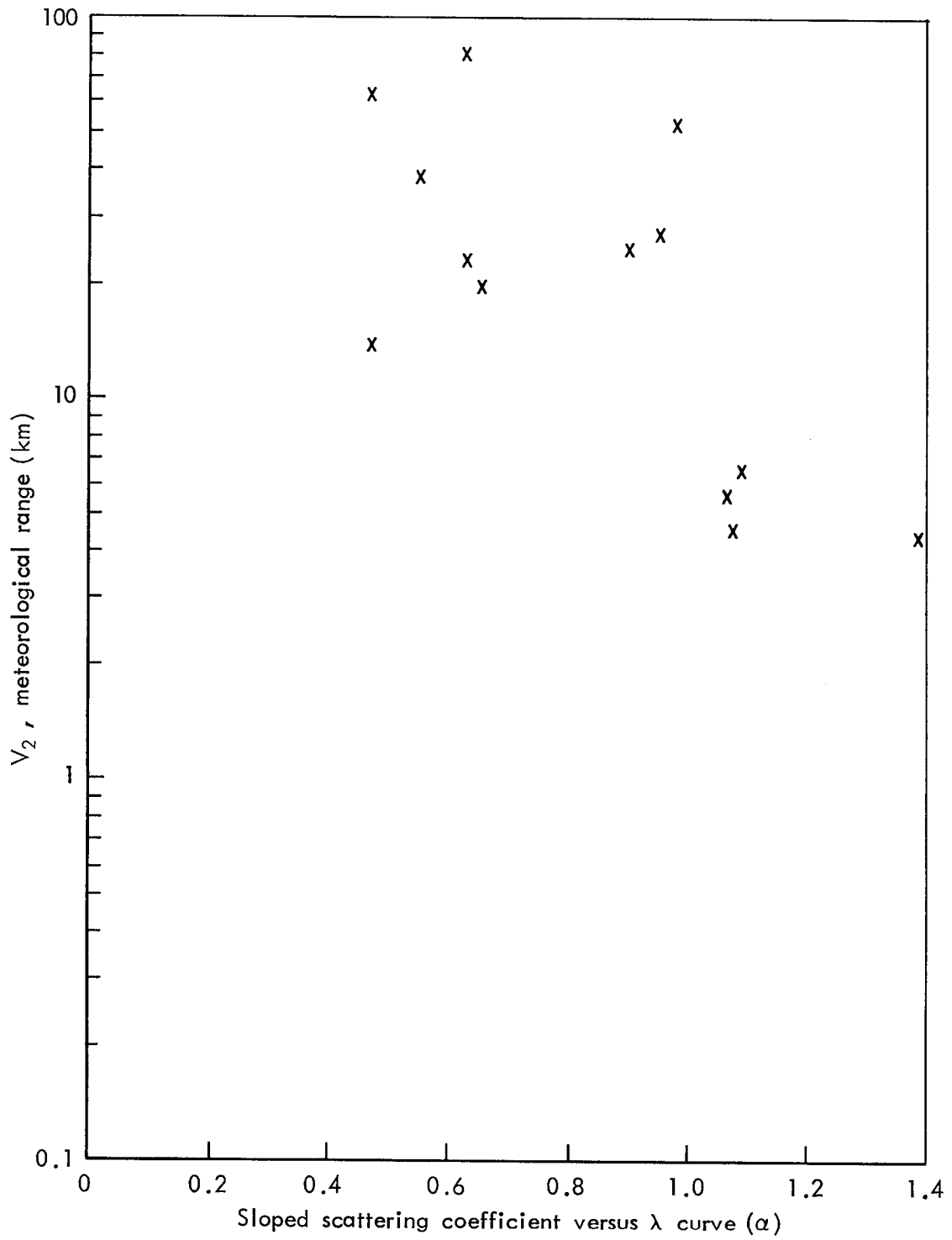
Fig. 14— Experimental values of slope of scattering coefficient curves
