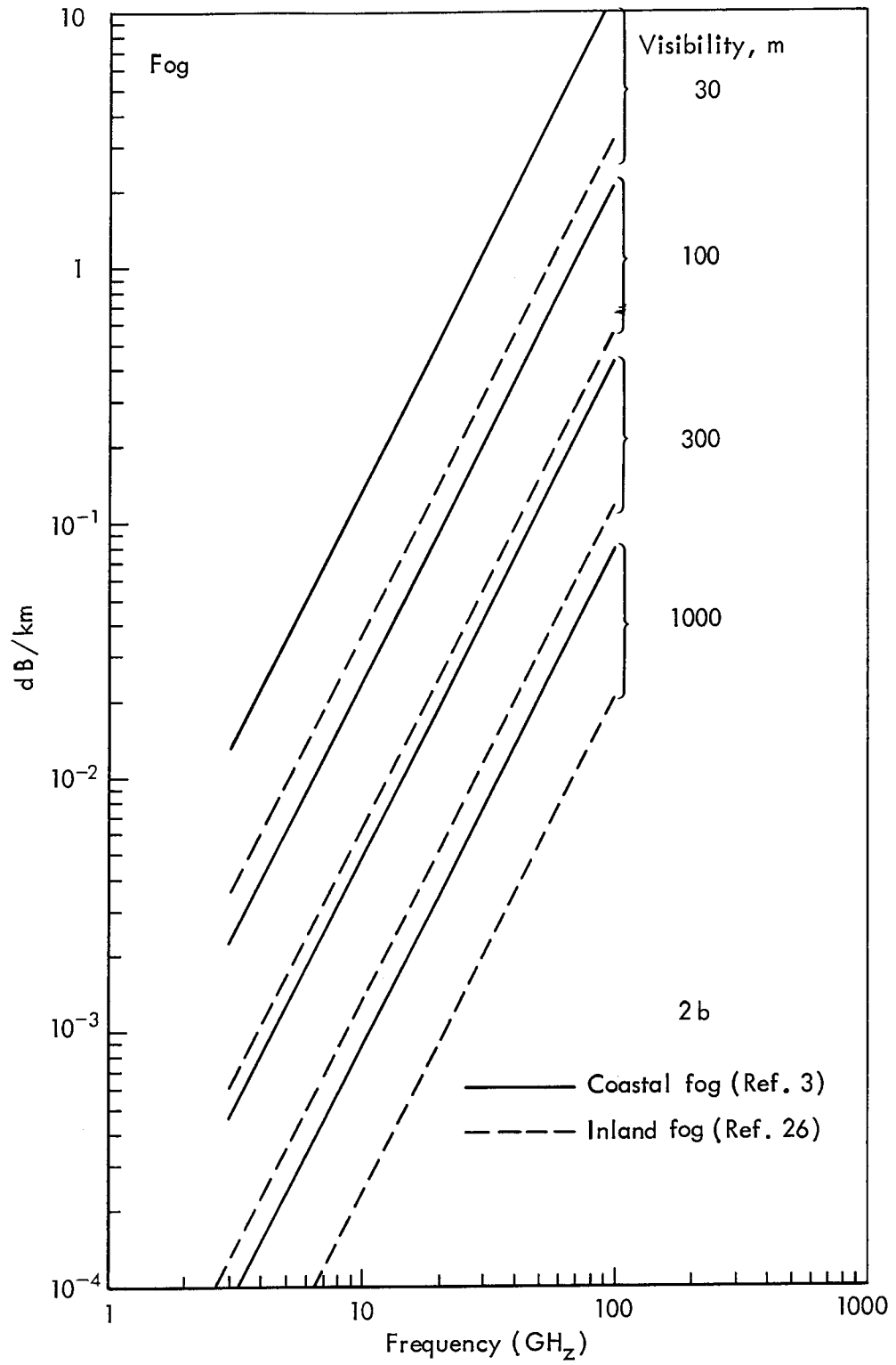
Fig. 12 — Calculated attenuation by fog at 18°C
