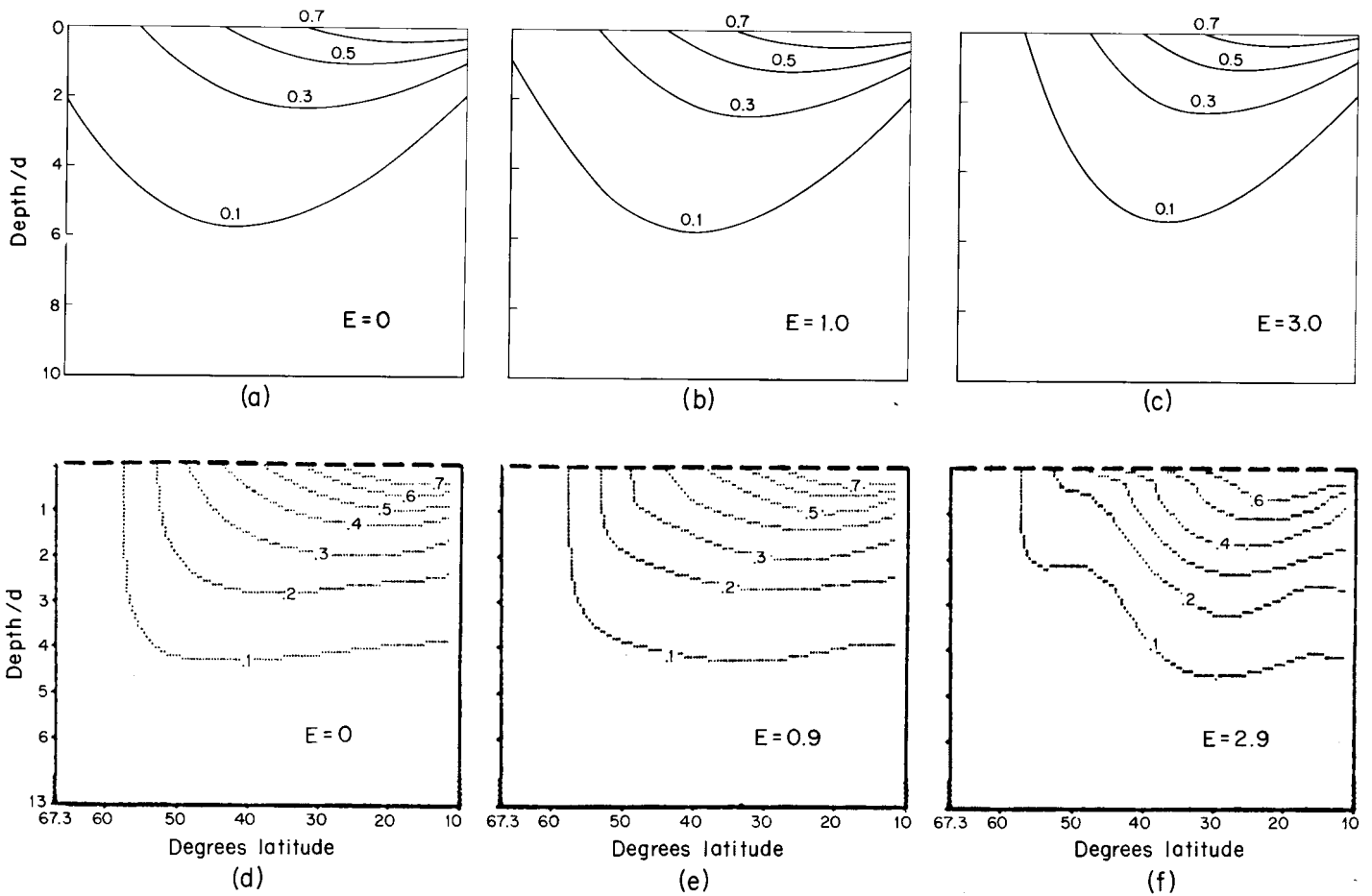
Fig. 4 -- North/south temperature sections bisecting the basin, (a through c) analytical model, (d through f) Bryan and Cox [1967]. From left to right E = 0 corresponds to no wind, E = 1 to moderate wind, and E = 3 to strong wind. The parameters K = 1 and C = 0.2 are held fixed.
