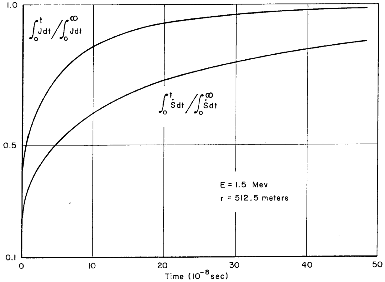
Fig. 5—Integrated Compton current and energy deposition as a function of time
