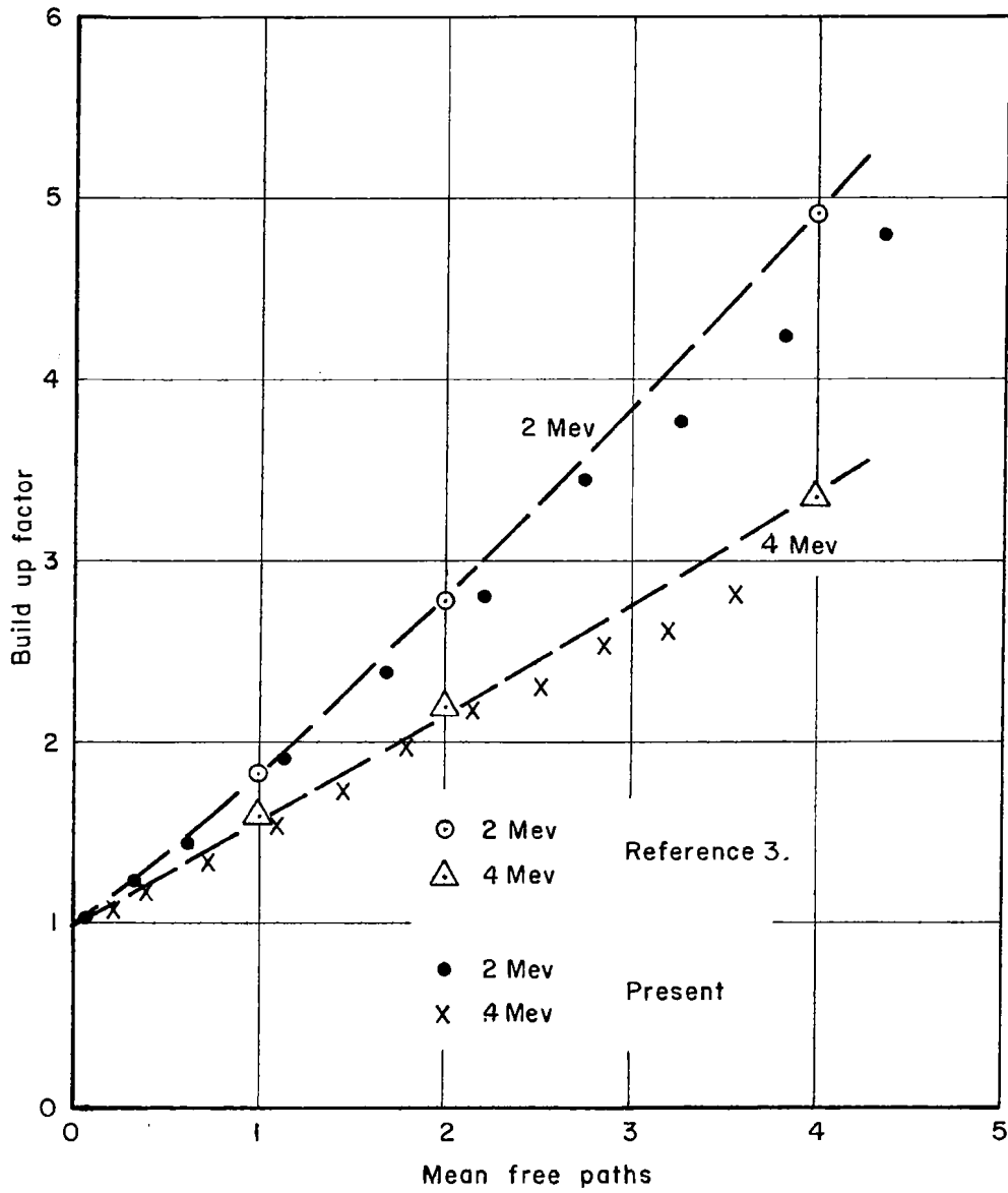
Fig. 14—Build up factor for energy deposition
