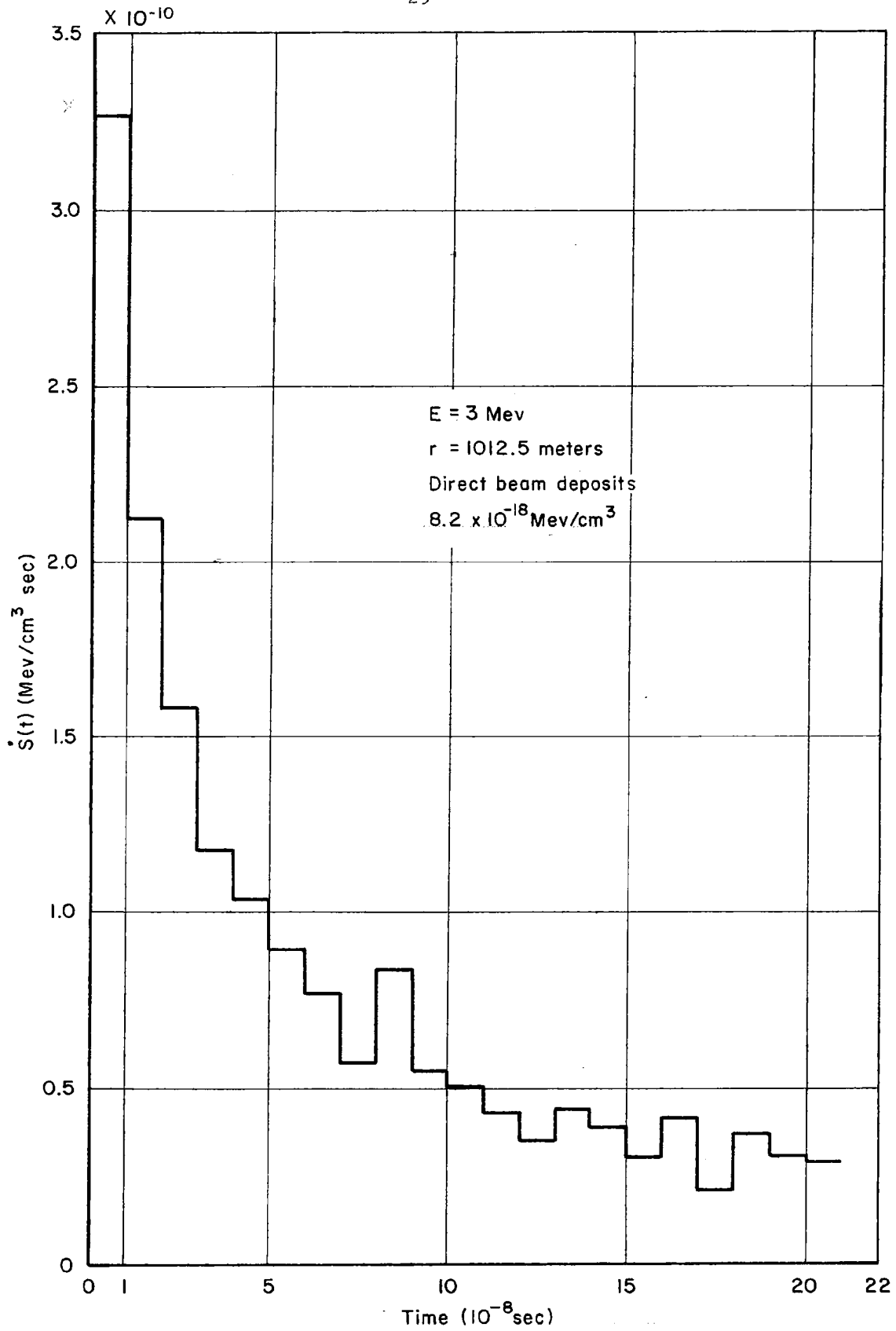
Fig. 3—Energy deposition rate as a function of time
