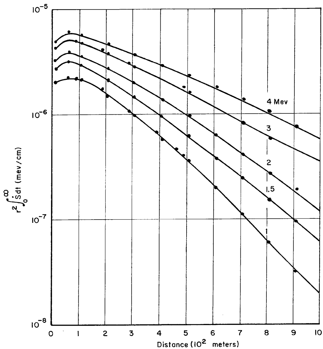
Fig. 9—Total energy deposition versus distance
