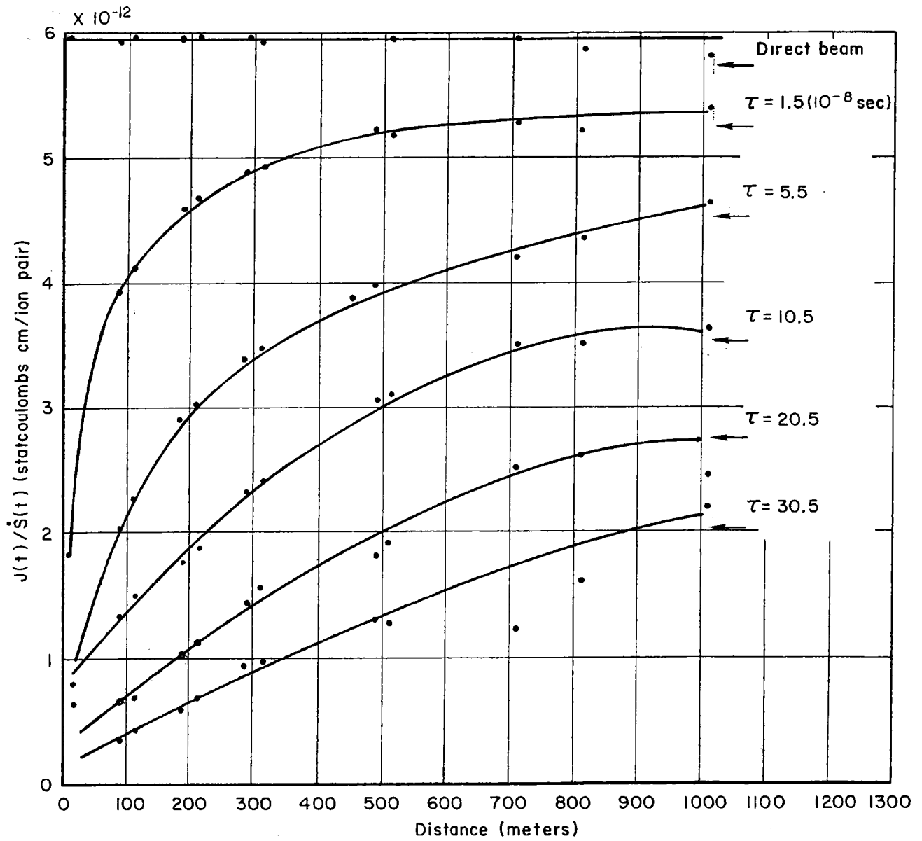
Fig. 8—Ratio of Compton current to energy deposition rate as a function of distance for a given delay time \tau . ( E = 3 \text{ Mev} )
