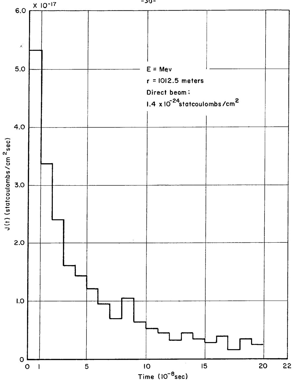
Fig. 4—Radial Compton current as a function of time
