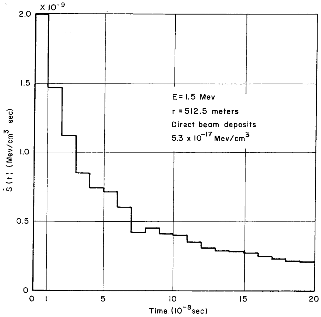
Fig. 1—Energy deposition rate as a function of time
