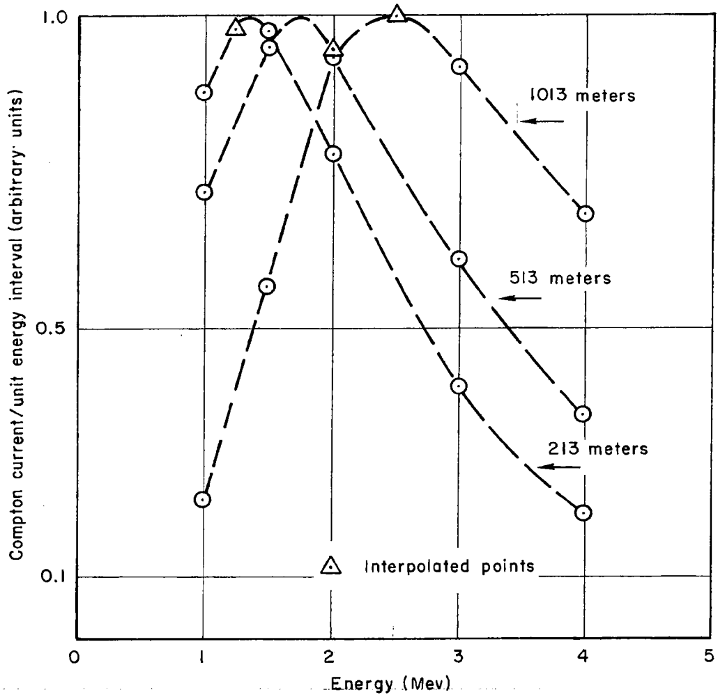
Fig. 12 — Compton current per unit energy interval for the Maienschein spectrum
