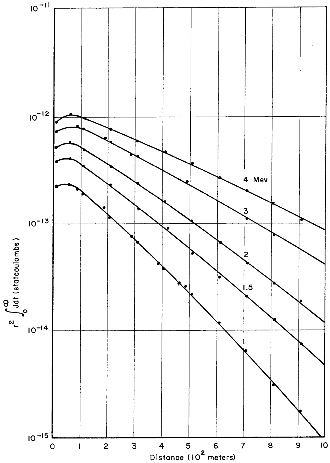
Fig. 10—Integrated radial Compton current versus distance
