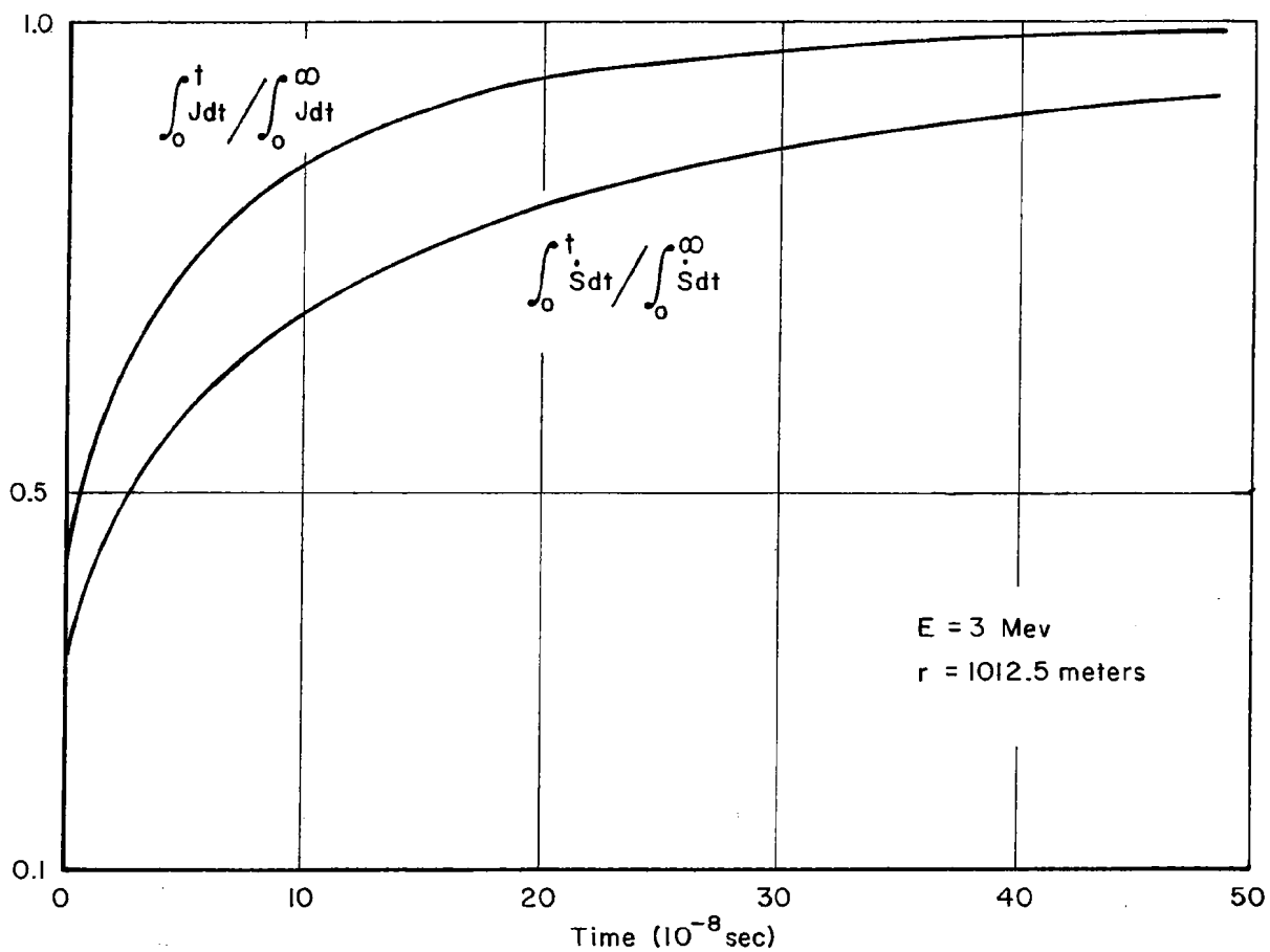
Fig. 6—Integrated Compton current and energy deposition as a function of time
