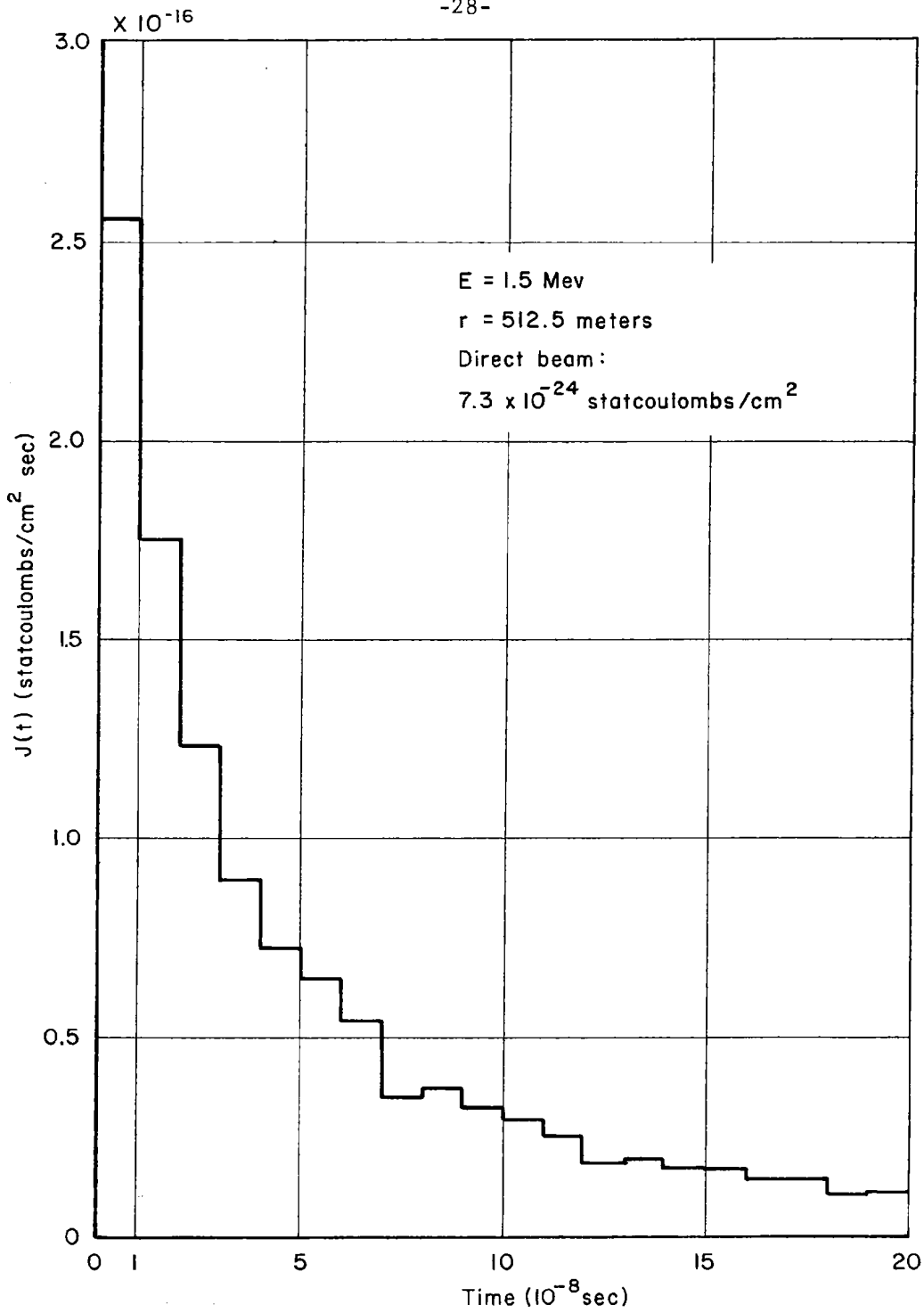
Fig. 2—Radial Compton current as a function of time
