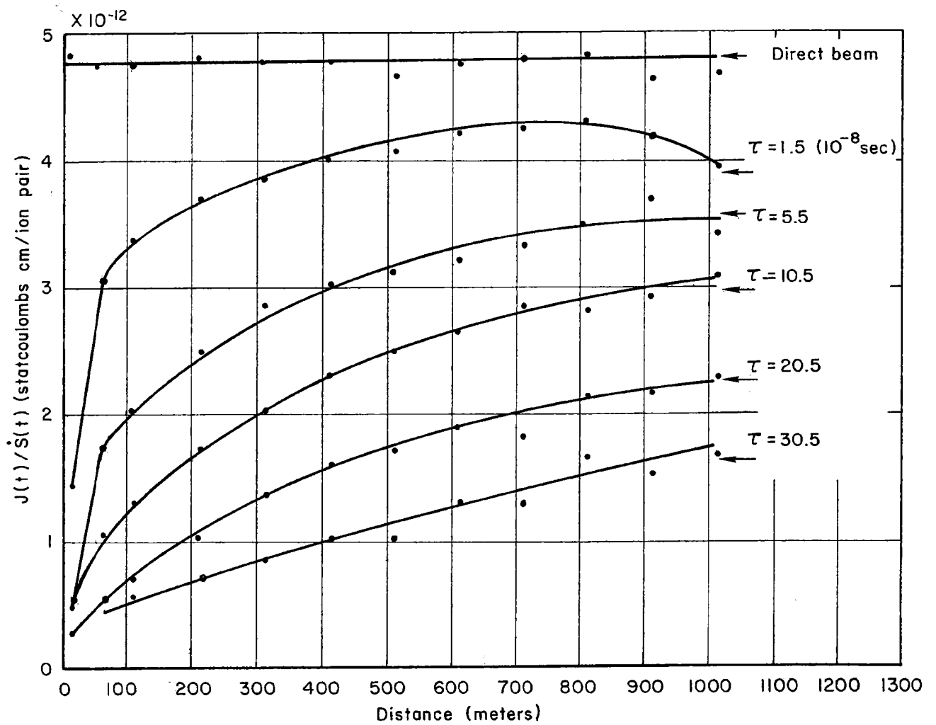
Fig. 7—Ratio of Compton current to energy deposition rate as a function of distance for a given delay time \tau . ( E=1.5 Mev)
