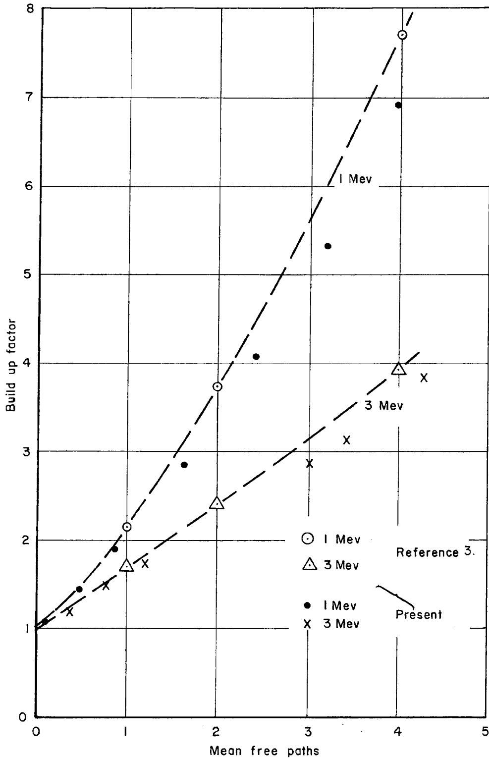
Fig. 13—Build up factor for energy deposition
