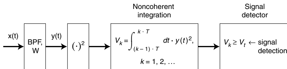
Figure 3.5—Energy Detector
